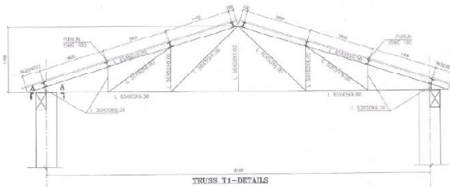
TRUSS T1-DETAILS
