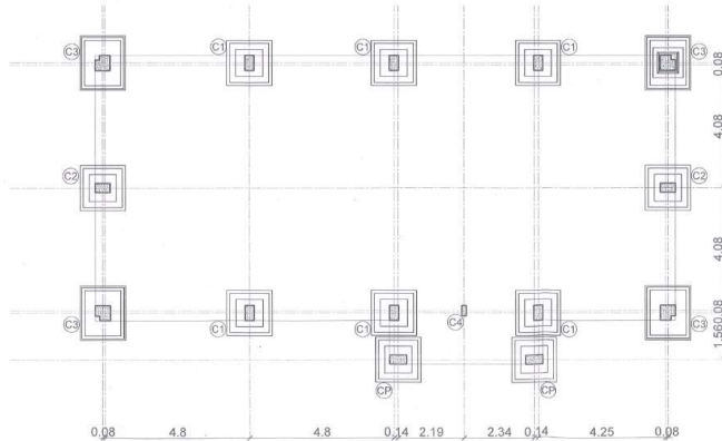
FOOTING PLAN SCALE 1:100
